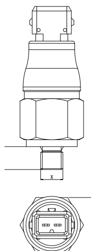
Connettore tipo AMP Junior power timer Connector type AMP Junior power timer
