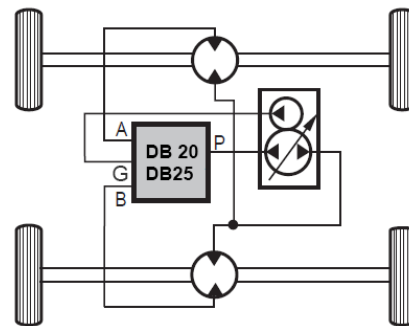
Flow divider operating as an axis separator with integrated pressure supply valves and supply port (S).
