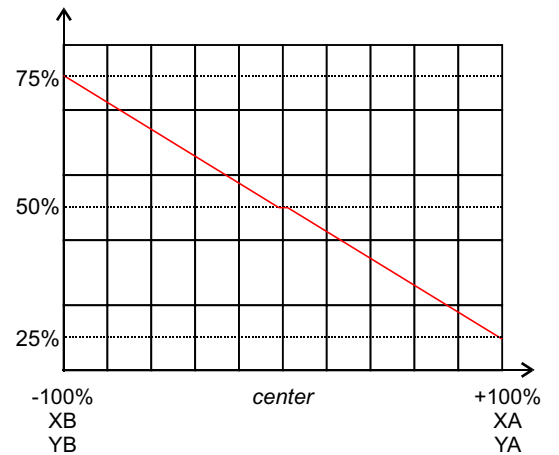
Output signal (V/Vsupply) for each axis
