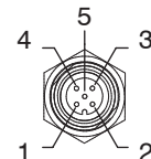
M12 5P MALE
