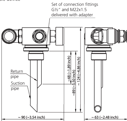
Suction-return adapter
